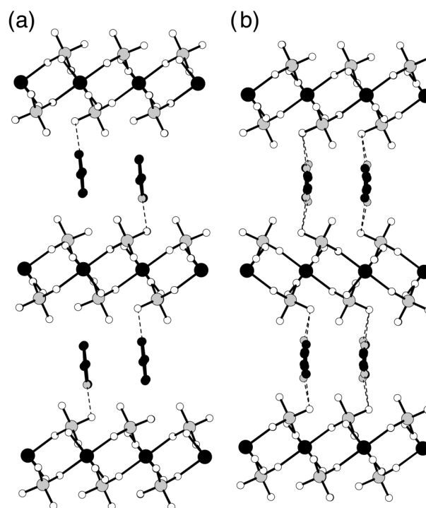
Fig. 5 Views of (a) compound I and (b) II , viewed along the crystallographic b axes, with the a axes running horizontally. Note the different orientations of the central inorganic layers in the two diagrams.
